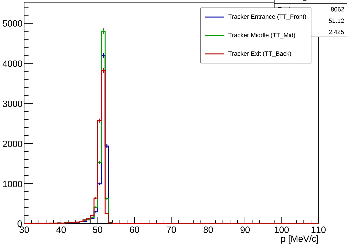
B2BCeEndpointDiffEnergy Reco Momentum at Tracker Entrance (TT_Front)
