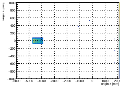
Monte Carlo truth: rank-0 trkmsim electron origins XZ
