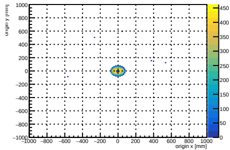
Monte Carlo truth: rank-0 trkmsim electron origins XY
