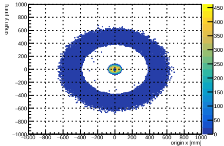
Monte Carlo truth: all trkmsim electron origins XY
