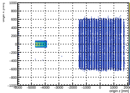
Monte Carlo truth: all trkmsim electron origins XZ
