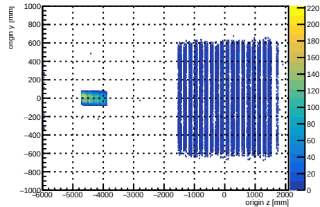
Monte Carlo truth: all trkmsim electron origins YZ
