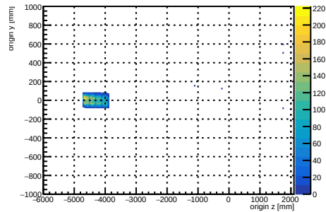
Monte Carlo truth: rank-0 trkmsim electron origins YZ
