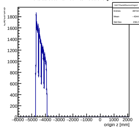
Monte Carlo truth: rank-0 trkmsim electron origins Z
