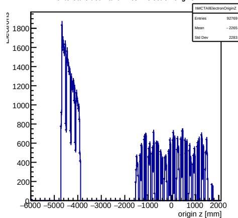
Monte Carlo truth: all trkmsim electron origins Z
