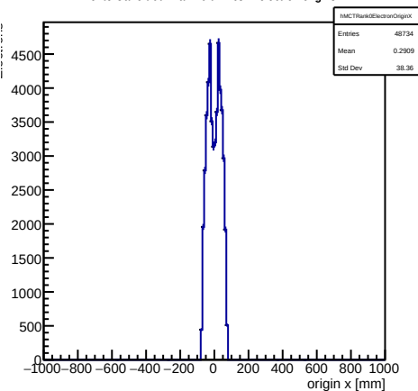
Monte Carlo truth: rank-0 trkmsim electron origins X
