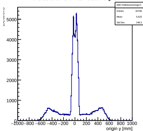
Monte Carlo truth: all trkmsim electron origins Y
