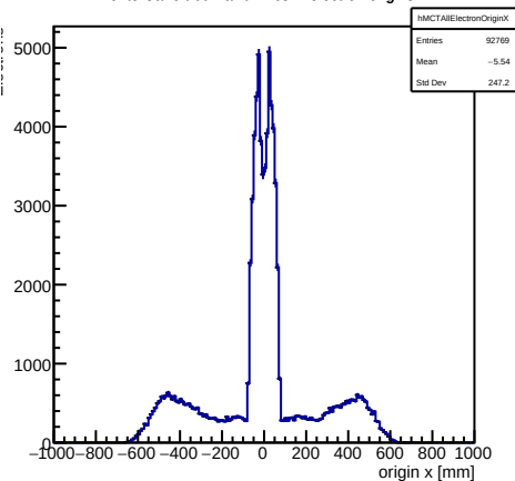
Monte Carlo truth: all trkmsim electron origins X
