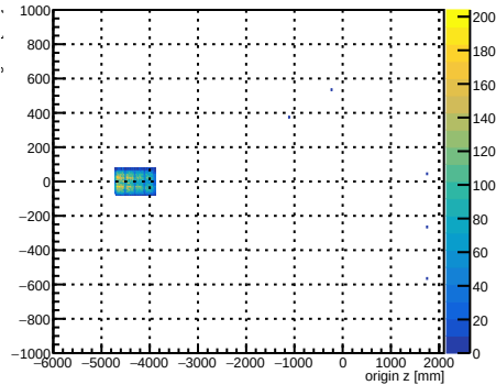
Monte Carlo truth: rank-0 trkmcsim electron origins XZ
