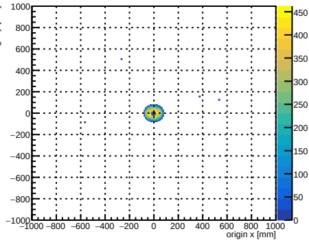
Monte Carlo truth: rank-0 trkmcsim electron origins XY
