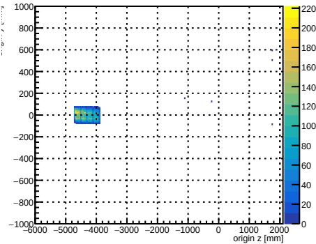
Monte Carlo truth: rank-0 trkmcsim electron origins YZ
