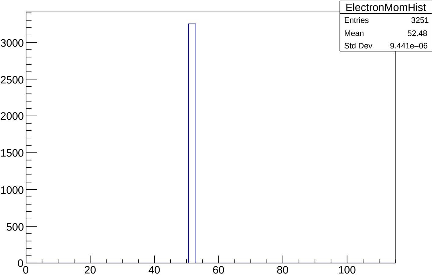
Momentum (MeV/c) of Electrons Produced by the Generator
