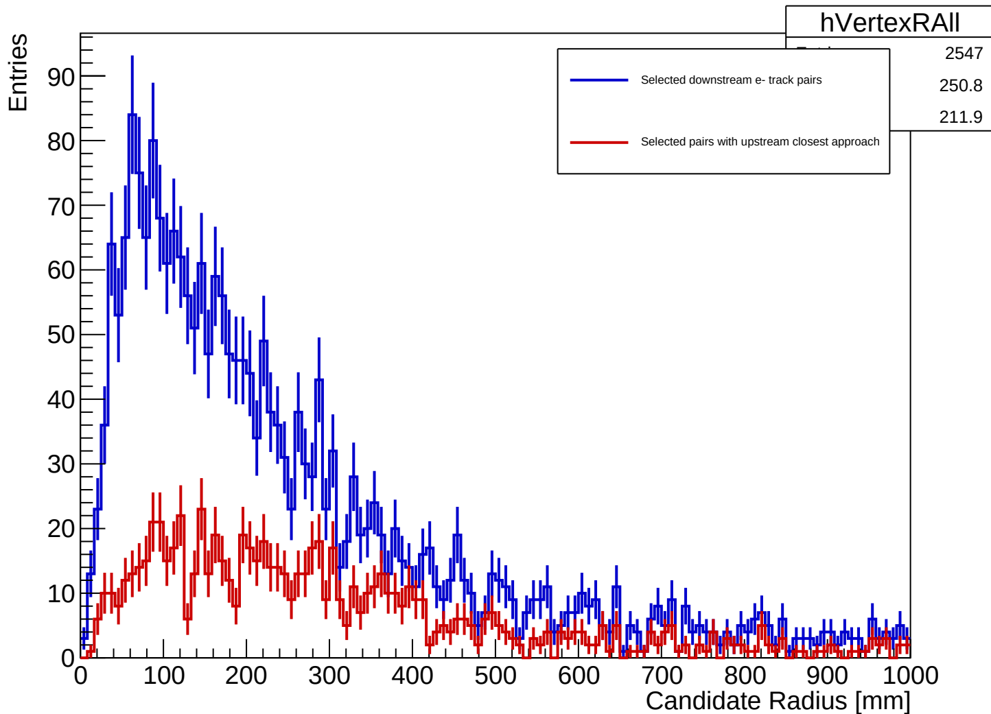
B2BCeEndpointDiffEnergy Downstream e- Candidate Common-Origin Radius
