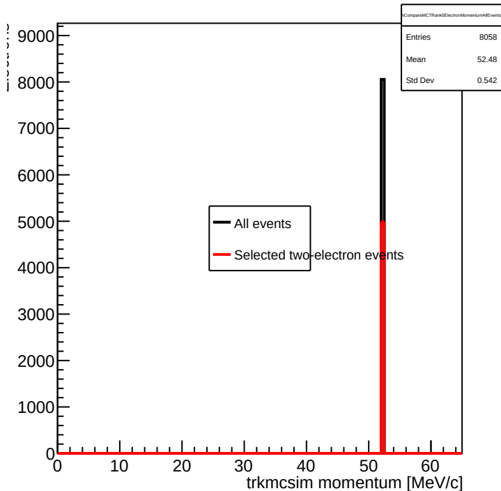
Monte Carlo truth rank-0 electrons: all events vs selected two-electron events
