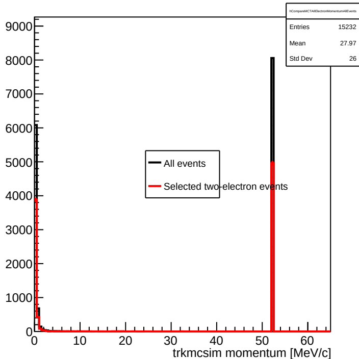
Monte Carlo truth all electrons: all events vs selected two-electron events
