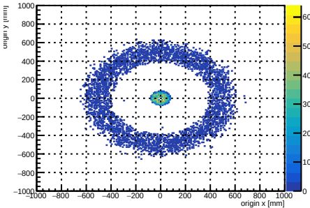
Monte Carlo truth: rank-0 trkmsim electron origins XY
