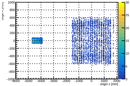
Monte Carlo truth: rank-0 trkmsim electron origins XZ
