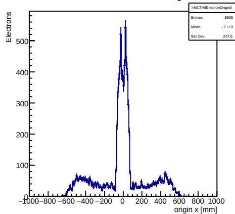
Monte Carlo truth: all trkmsim electron origins X
