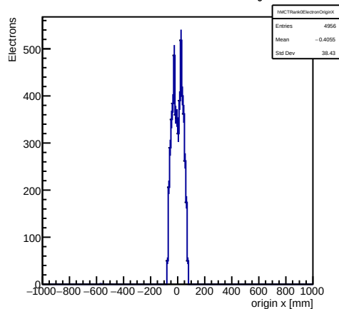
Monte Carlo truth: rank-0 trkmsim electron origins X
