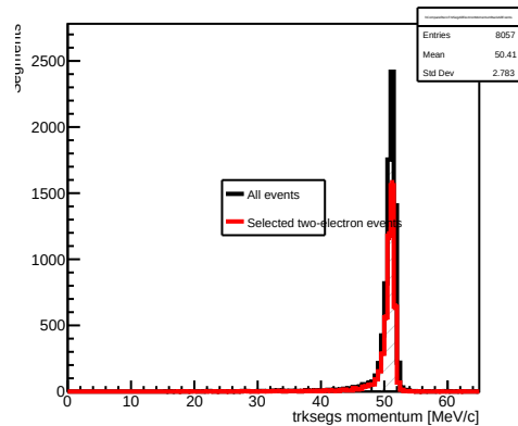
All electron-matched trksegs at TT_Back: all events vs selected two-electron events
