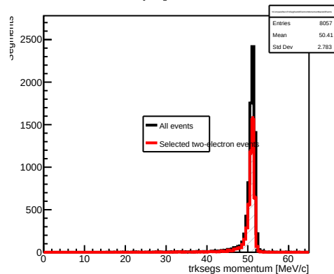
Rank-0 electron-matched trksegs at TT_Back: all events vs selected two-electron events
