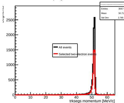
Rank-0 electron-matched trksegs at TT_Mid: all events vs selected two-electron events
