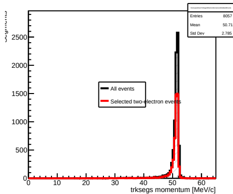
All electron-matched trksegs at TT_Mid: all events vs selected two-electron events
