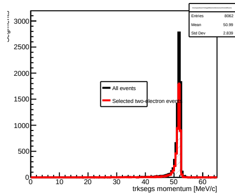
All electron-matched trksegs at TT_Front: all events vs selected two-electron events
