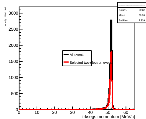
Rank-0 electron-matched trksegs at TT_Front: all events vs selected two-electron events
