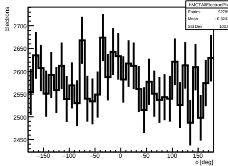
Monte Carlo truth: all trkmcsim electron \phi
