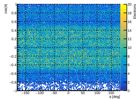
Monte Carlo truth: all trkmcsim electron \cos(\theta) vs \phi
