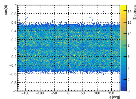
Monte Carlo truth: rank-0 trkmcsim electron \cos(\theta) vs \phi
