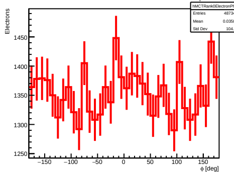
Monte Carlo truth: rank-0 trkmcsim electron \phi
