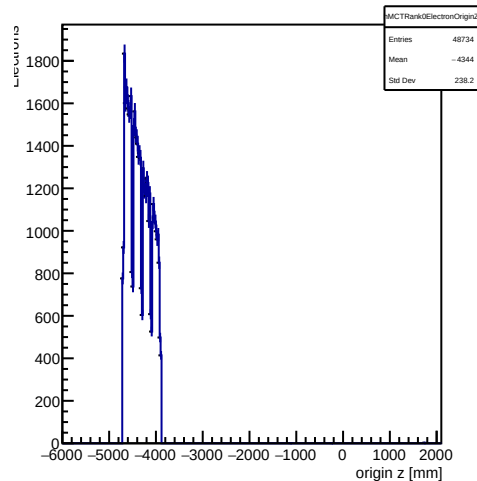
Monte Carlo truth: rank-0 trkmcsim electron origins Z
