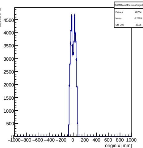
Monte Carlo truth: rank-0 trkmcsim electron origins X
