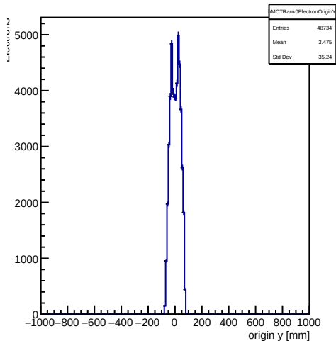
Monte Carlo truth: rank-0 trkmcsim electron origins Y
