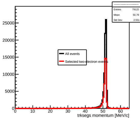
All electron-matched trksegs at TT_Mid: all events vs selected two-electron events
