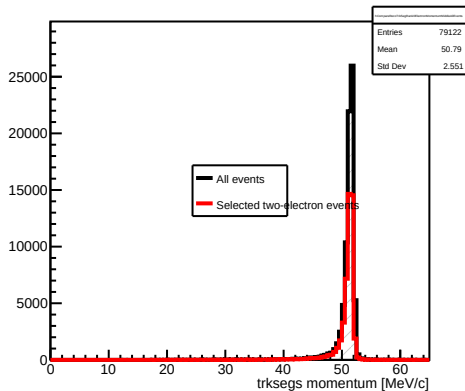
Rank-0 electron-matched trksegs at TT_Mid: all events vs selected two-electron events
