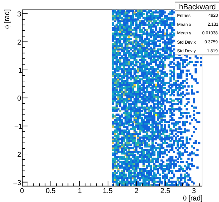
Backward electrons
