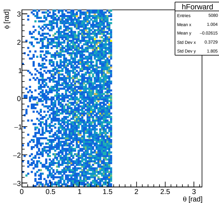
Forward electrons
