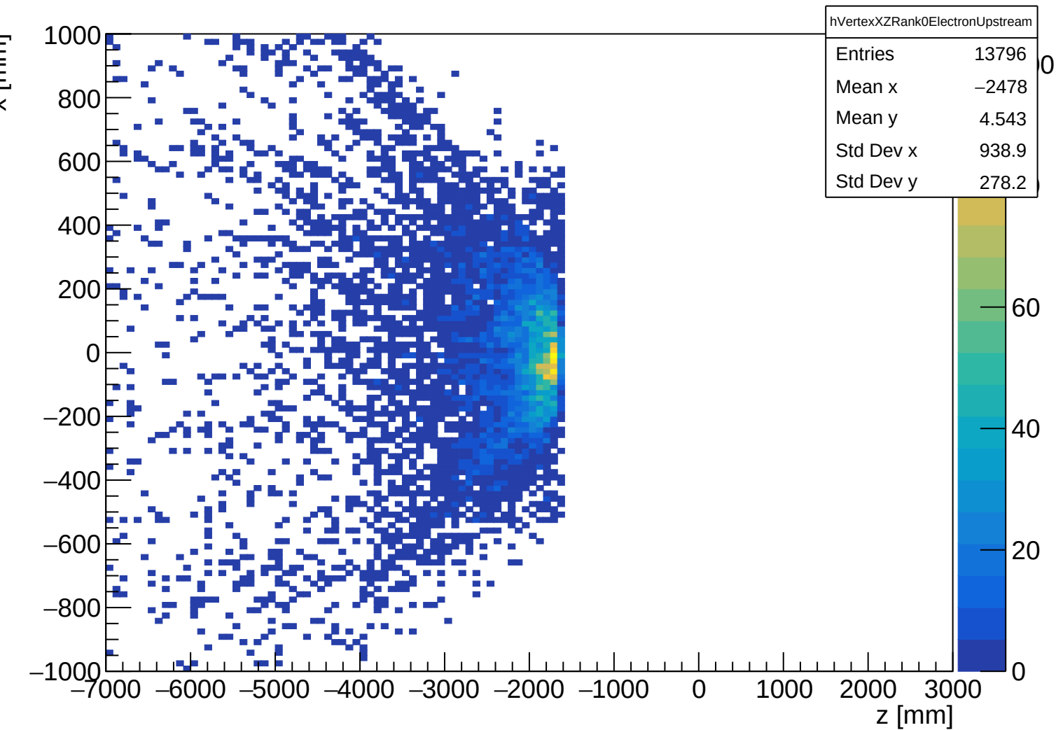
B2BCeEndpointDiffEnergy Candidate Common-Origin Map for Rank-0 Electron Track Pairs (Upstream Only)
