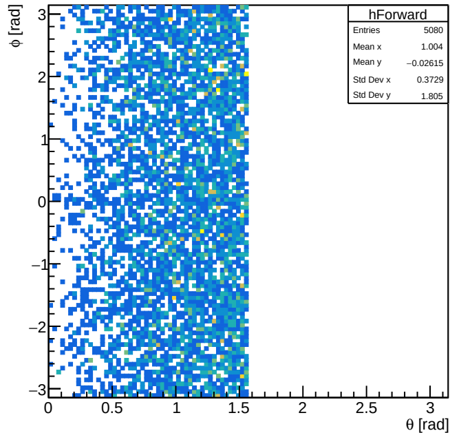
Forward electrons
