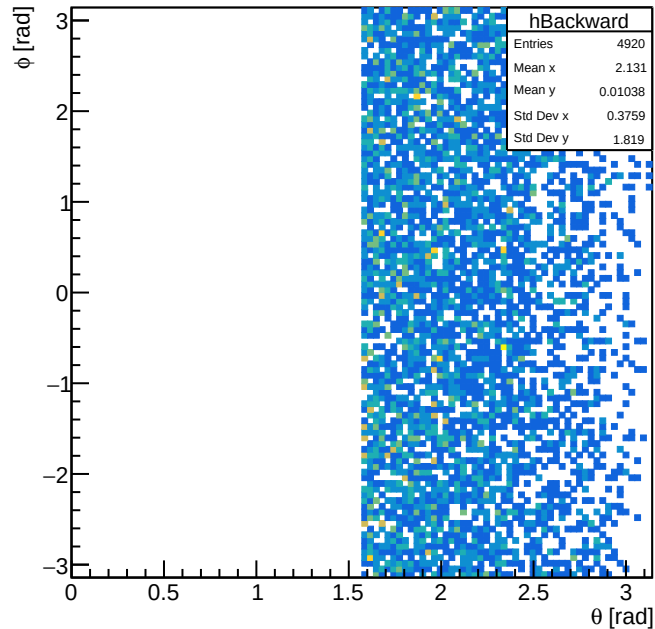
Backward electrons
