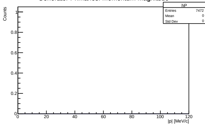
Generator Primaries: Momentum Magnitude
