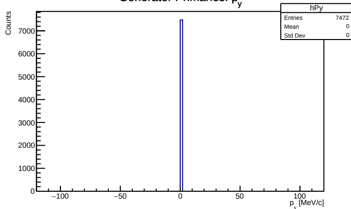
Generator Primaries: p_y
