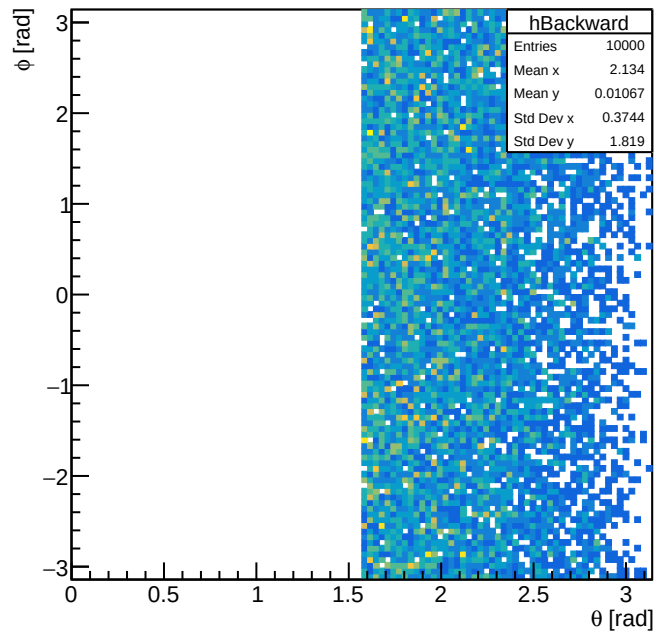
Backward electrons
