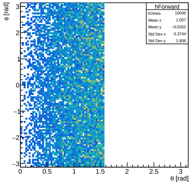
Forward electrons
