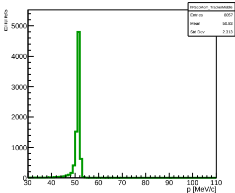
B2BCeEndpointDiffEnergy Reco Momentum at Tracker Middle (TT_Mid)
