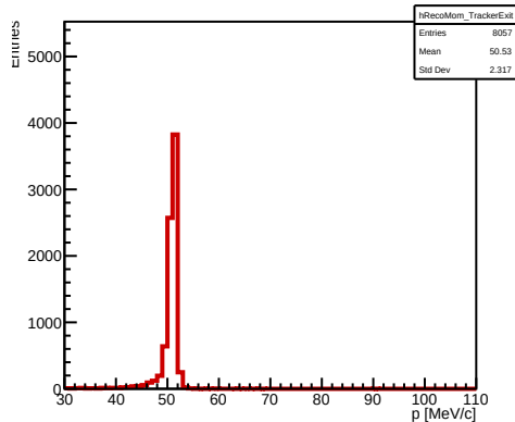
B2BCeEndpointDiffEnergy Reco Momentum at Tracker Exit (TT_Back)
