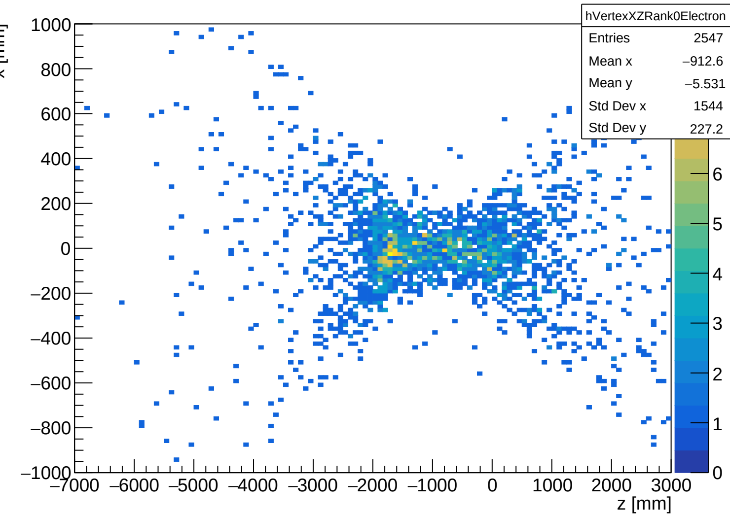
B2BCeEndpointDiffEnergy Candidate Common-Origin Map for Rank-0 Electron Track Pairs
