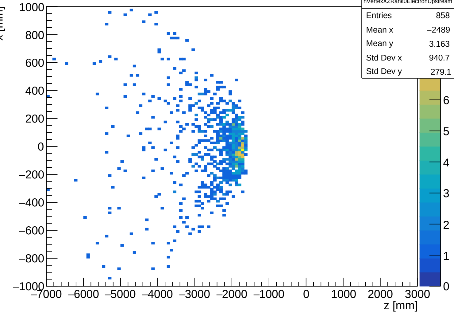
B2BCeEndpointDiffEnergy Candidate Common-Origin Map for Rank-0 Electron Track Pairs (Upstream Only)
