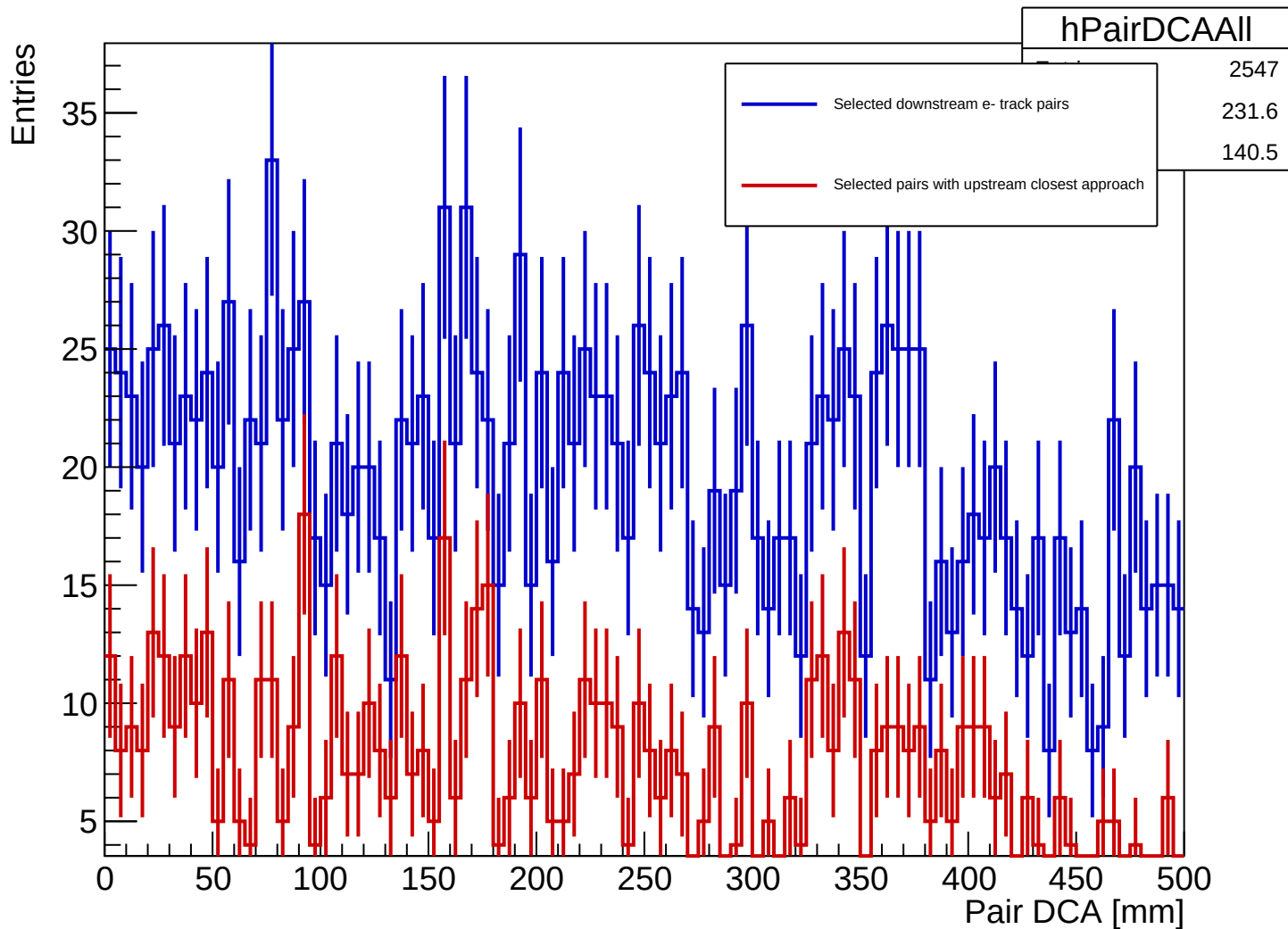
B2BCeEndpointDiffEnergy Downstream e- Pair DCA from Backward Extrapolation
