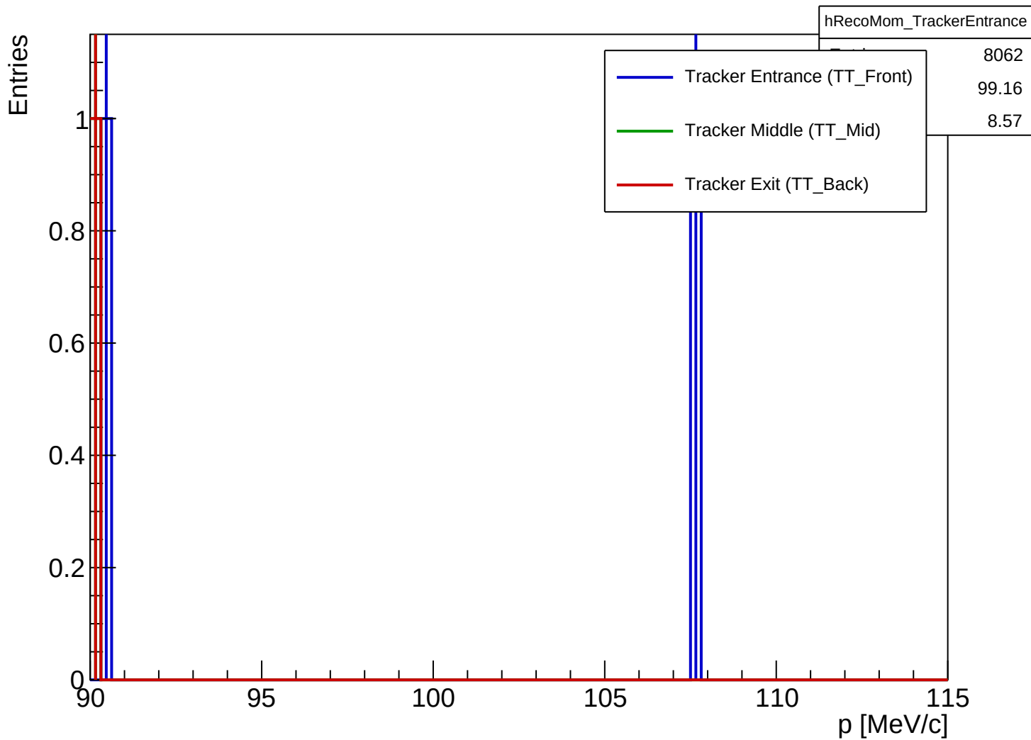
B2BCeEndpointDiffEnergy Reco Momentum at Tracker Entrance (TT_Front)
