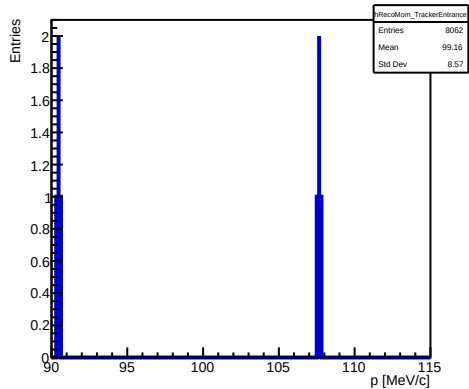
B2BCeEndpointDiffEnergy Reco Momentum at Tracker Entrance (TT_Front)
