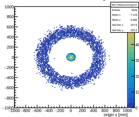
Monte Carlo truth: all trkmsim electron origins XY
