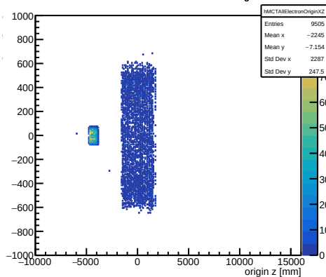
Monte Carlo truth: all trkmsim electron origins XZ
