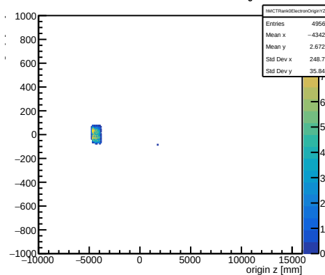
Monte Carlo truth: rank-0 trkmsim electron origins YZ
