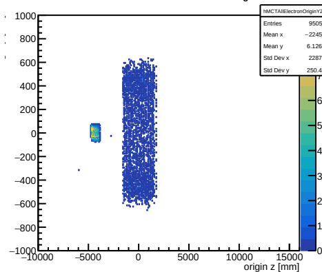
Monte Carlo truth: all trkmsim electron origins YZ
