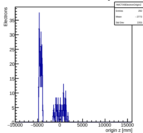
Monte Carlo truth: all trkmsim electron origins Z
