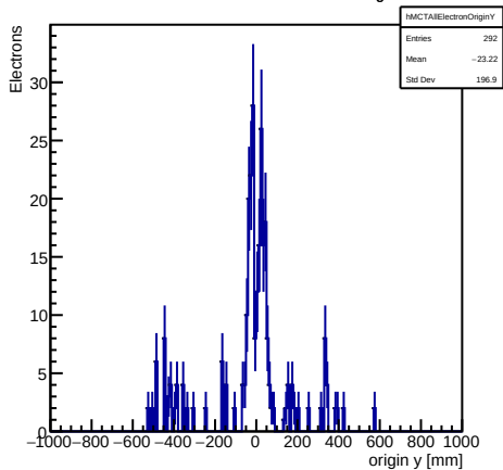
Monte Carlo truth: all trkmsim electron origins Y
