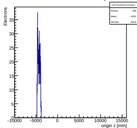
Monte Carlo truth: rank-0 trkmsim electron origins Z
