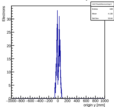
Monte Carlo truth: rank-0 trkmsim electron origins Y
