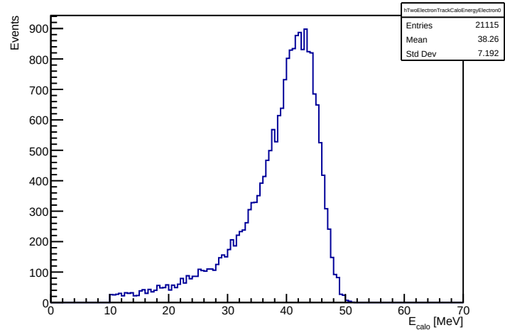
Two-track events: electron 0 calorimeter energy
