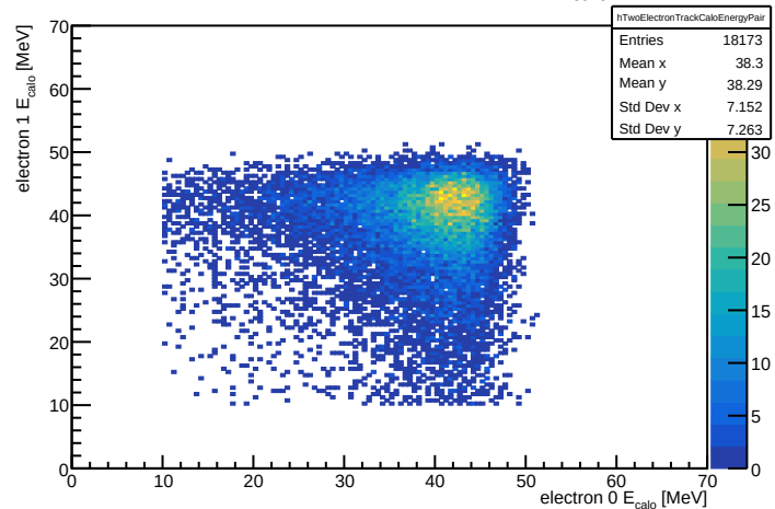
Two-track events: electron calorimeter energy pair
