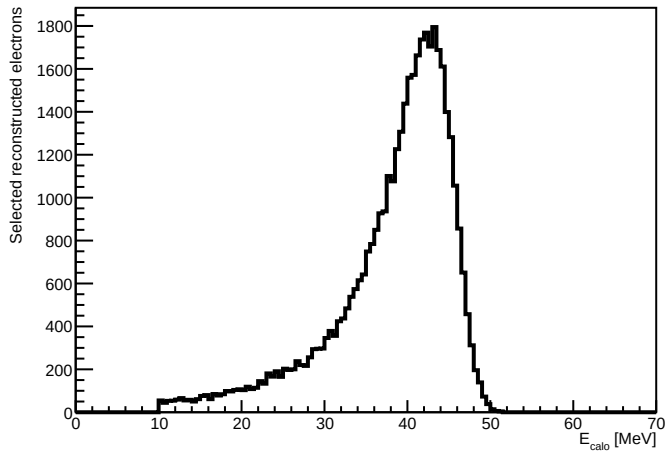
Two-track events: electron 1 calorimeter energy
