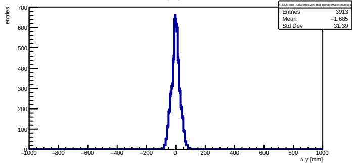
TEST: foil-index matched minimum- |\Delta t| vertex minus truth origin y difference
