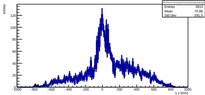
TEST: foil-index matched minimum- |\Delta t| vertex minus truth origin z difference
