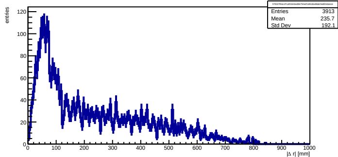
TEST: foil-index matched minimum- |\Delta t| vertex minus truth origin residual magnitude
