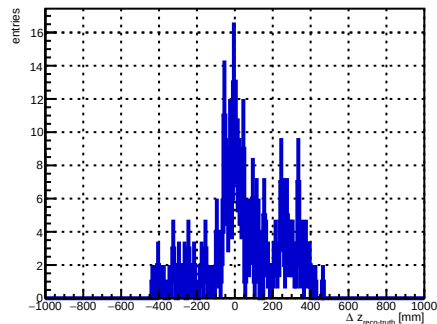
selected foil index 17, N = 245
