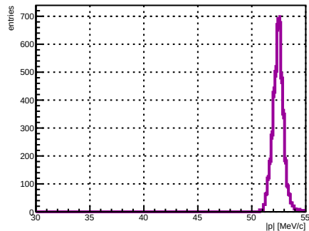
Selected track ST_Foils intersection |p|, foil index 12, N = 4446
