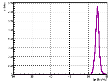
Selected track ST_Foils intersection |p|, foil index 17, N = 4709
