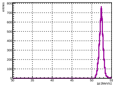
Selected track ST_Foils intersection |p|, foil index 16, N = 4583
