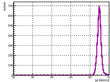
Selected track ST_Foils intersection |p|, foil index 14, N = 4571
