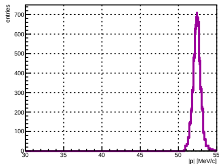
Selected track ST_Foils intersection |p|, foil index 15, N = 4504
