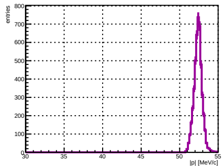
Selected track ST_Foils intersection |p|, foil index 18, N = 4745
