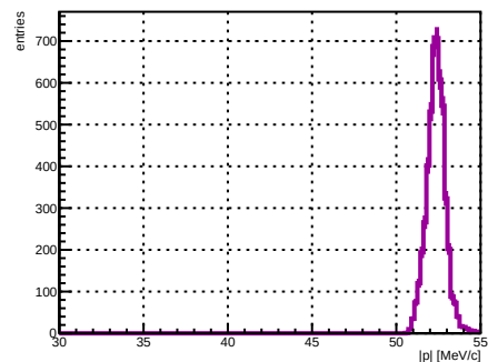
Selected track ST_Foils intersection |p|, foil index 23, N = 4989
