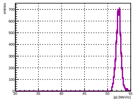
Selected track ST_Foils intersection |p|, foil index 21, N = 4936
