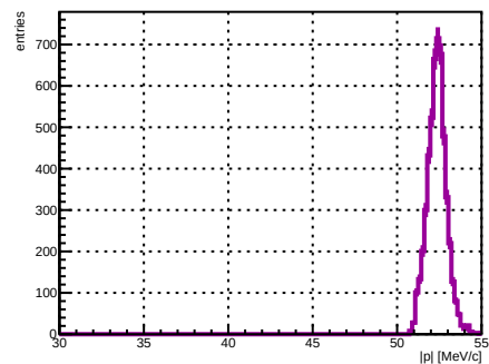
Selected track ST_Foils intersection |p|, foil index 26, N = 5148
