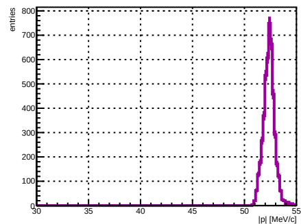
Selected track ST_Foils intersection |p|, foil index 20, N = 4784
