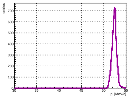
Selected track ST_Foils intersection |p|, foil index 19, N = 4718
