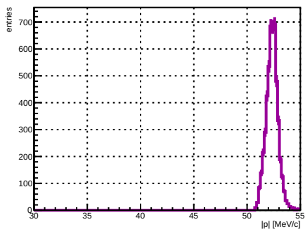
Selected track ST_Foils intersection |p|, foil index 25, N = 5098
