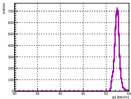
Selected track ST_Foils intersection |p|, foil index 22, N = 5019
