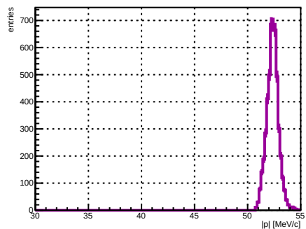
Selected track ST_Foils intersection |p|, foil index 24, N = 4981
