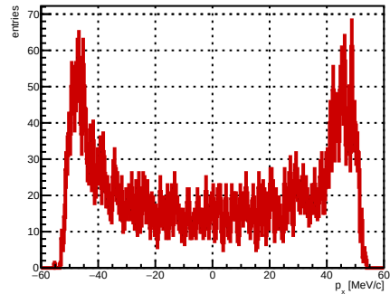
Selected track ST_Foils intersection p_x , foil index 14, N = 4571
