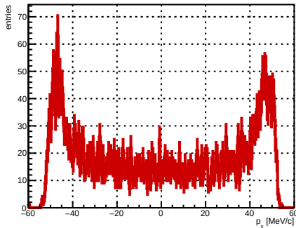
Selected track ST_Foils intersection p_x , foil index 9, N = 4224
