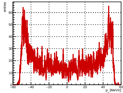
Selected track ST_Foils intersection p_x , foil index 11, N = 4296
