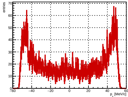
Selected track ST_Foils intersection p_x , foil index 10, N = 4403
