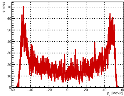
Selected track ST_Foils intersection p_x , foil index 12, N = 4446
