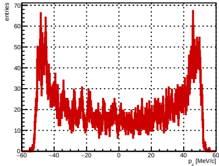
Selected track ST_Foils intersection p_x , foil index 16, N = 4583
