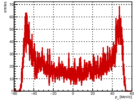
Selected track ST_Foils intersection p_x , foil index 17, N = 4709
