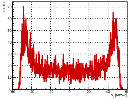
Selected track ST_Foils intersection p_x , foil index 15, N = 4504
