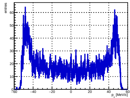
Selected track ST_Foils intersection p_y , foil index 11, N = 4296
