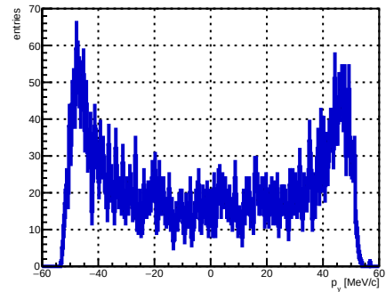
Selected track ST_Foils intersection p_y , foil index 17, N = 4709
