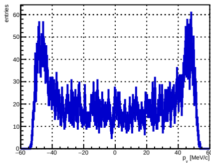
Selected track ST_Foils intersection p_y , foil index 15, N = 4504
