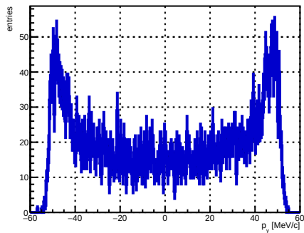
Selected track ST_Foils intersection p_y , foil index 10, N = 4403
