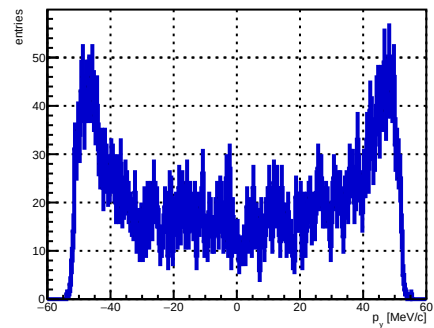
Selected track ST_Foils intersection p_y , foil index 14, N = 4571
