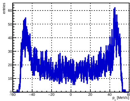
Selected track ST_Foils intersection p_y , foil index 12, N = 4446
