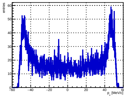
Selected track ST_Foils intersection p_y , foil index 9, N = 4224
