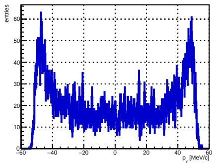
Selected track ST_Foils intersection p_y , foil index 13, N = 4502
