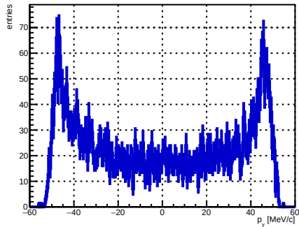
Selected track ST_Foils intersection p_y , foil index 25, N = 5098
