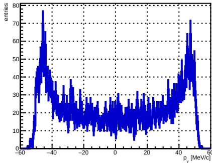
Selected track ST_Foils intersection p_y , foil index 24, N = 4981
