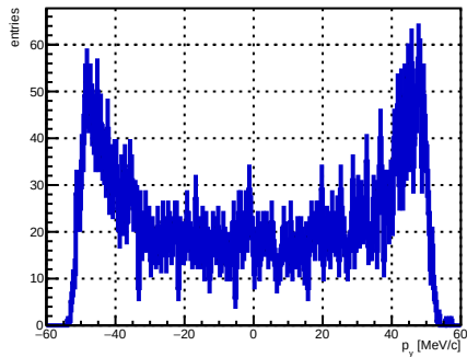
Selected track ST_Foils intersection p_y , foil index 22, N = 5019
