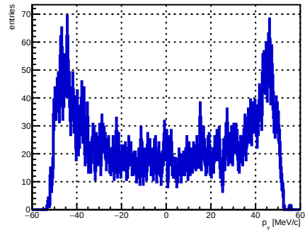
Selected track ST_Foils intersection p_y , foil index 26, N = 5148
