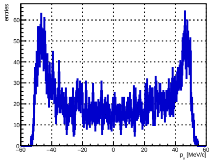
Selected track ST_Foils intersection p_y , foil index 19, N = 4718
