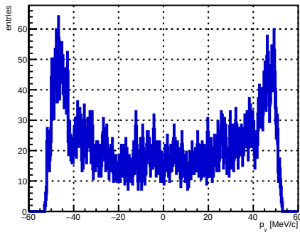
Selected track ST_Foils intersection p_y , foil index 18, N = 4745
