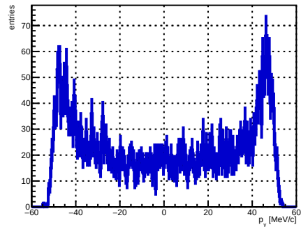
Selected track ST_Foils intersection p_y , foil index 23, N = 4989
