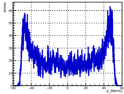
Selected track ST_Foils intersection p_y , foil index 20, N = 4784
