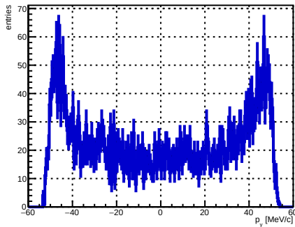
Selected track ST_Foils intersection p_y , foil index 21, N = 4936
