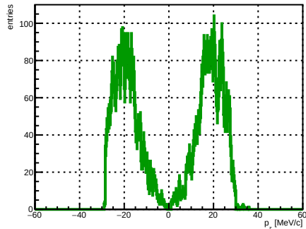
Selected track ST_Foils intersection p_x , foil index 24, N = 4981
