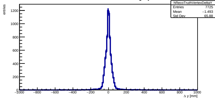
Selected two-track vertex minus truth origin y difference
