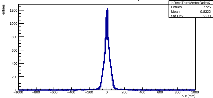
Selected two-track vertex minus truth origin x difference
