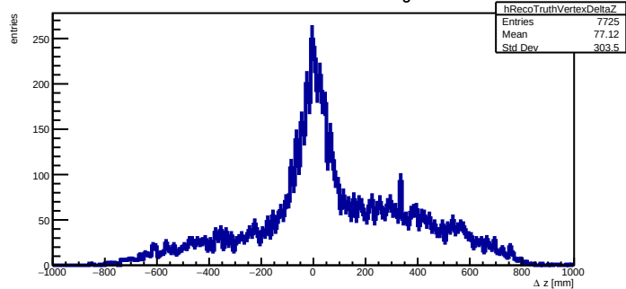
Selected two-track vertex minus truth origin z difference
