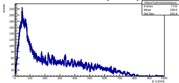
Selected two-track vertex minus truth origin residual magnitude
