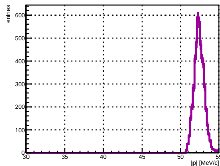
Selected track ST_Foils intersection |p|, foil index 32, N = 4920
