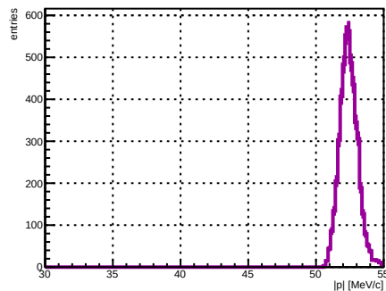
Selected track ST_Foils intersection |p|, foil index 33, N = 4938
