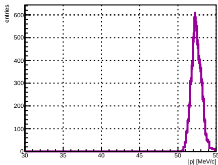
Selected track ST_Foils intersection |p|, foil index 34, N = 4972
