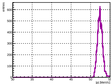
Selected track ST_Foils intersection |p|, foil index 31, N = 4961
