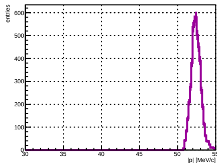
Selected track ST_Foils intersection |p|, foil index 30, N = 4938
