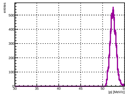
Selected track ST_Foils intersection |p|, foil index 35, N = 4836
