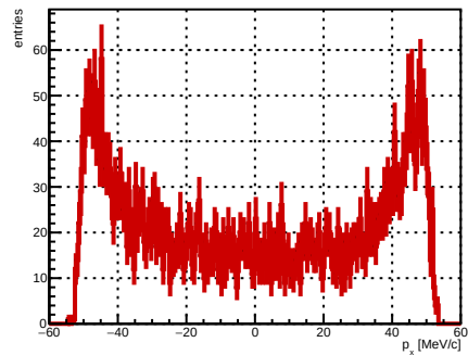
Selected track ST_Foils intersection p_x , foil index 17, N = 4698
