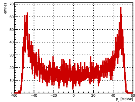
Selected track ST_Foils intersection p_x , foil index 11, N = 4350
