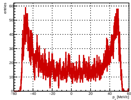
Selected track ST_Foils intersection p_x , foil index 14, N = 4320
