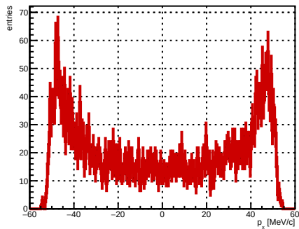
Selected track ST_Foils intersection p_x , foil index 16, N = 4494
