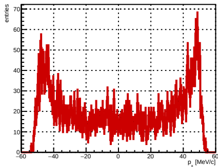
Selected track ST_Foils intersection p_x , foil index 15, N = 4426
