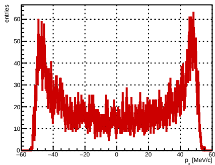
Selected track ST_Foils intersection p_x , foil index 13, N = 4387
