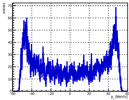
Selected track ST_Foils intersection p_y , foil index 15, N = 4426
