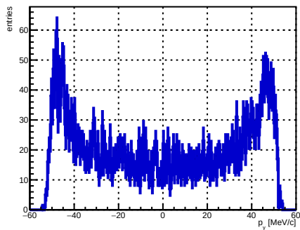
Selected track ST_Foils intersection p_y , foil index 16, N = 4494
