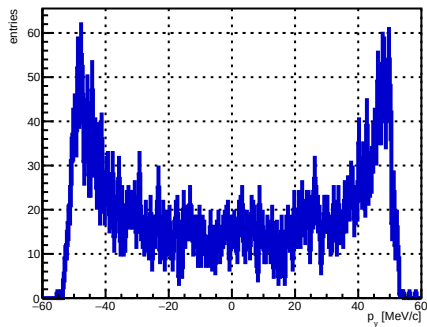
Selected track ST_Foils intersection p_y , foil index 10, N = 4281
