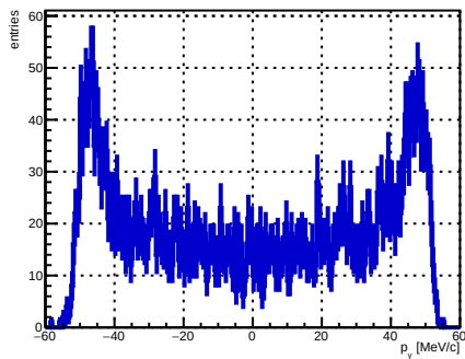
Selected track ST_Foils intersection p_y , foil index 12, N = 4314
