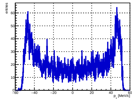
Selected track ST_Foils intersection p_y , foil index 17, N = 4698
