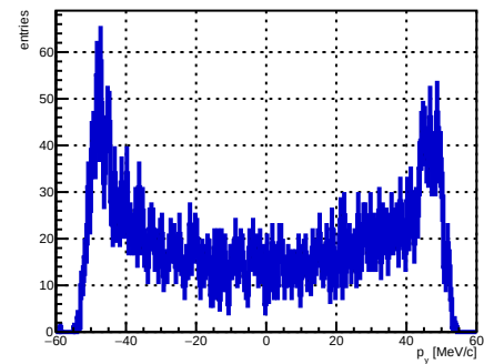
Selected track ST_Foils intersection p_y , foil index 14, N = 4320
