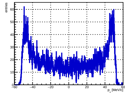
Selected track ST_Foils intersection p_y , foil index 11, N = 4350
