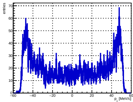
Selected track ST_Foils intersection p_y , foil index 13, N = 4387
