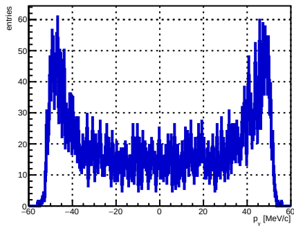
Selected track ST_Foils intersection p_y , foil index 9, N = 4323
