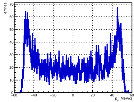
Selected track ST_Foils intersection p_y , foil index 23, N = 4878
