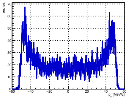
Selected track ST_Foils intersection p_y , foil index 21, N = 4803
