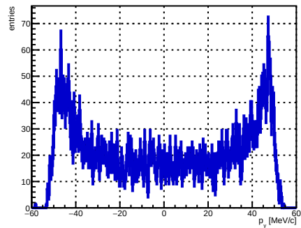
Selected track ST_Foils intersection p_y , foil index 20, N = 4757
