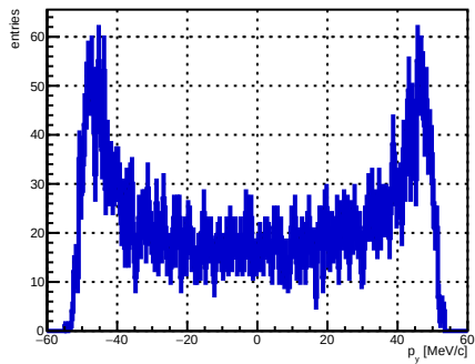
Selected track ST_Foils intersection p_y , foil index 25, N = 4880
