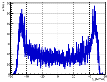
Selected track ST_Foils intersection p_y , foil index 22, N = 4812
