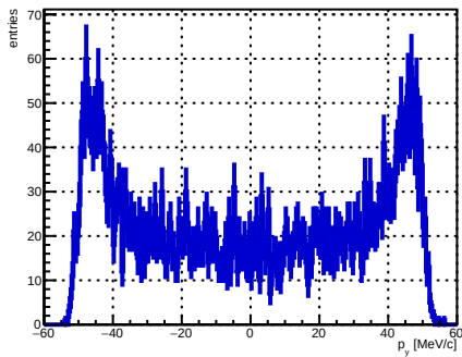
Selected track ST_Foils intersection p_y , foil index 24, N = 4944
