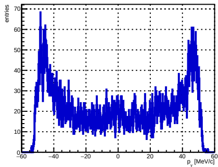
Selected track ST_Foils intersection p_y , foil index 19, N = 4803
