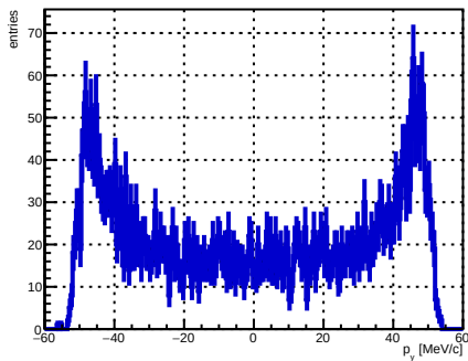
Selected track ST_Foils intersection p_y , foil index 18, N = 4740
