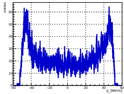
Selected track ST_Foils intersection p_y , foil index 26, N = 5042
