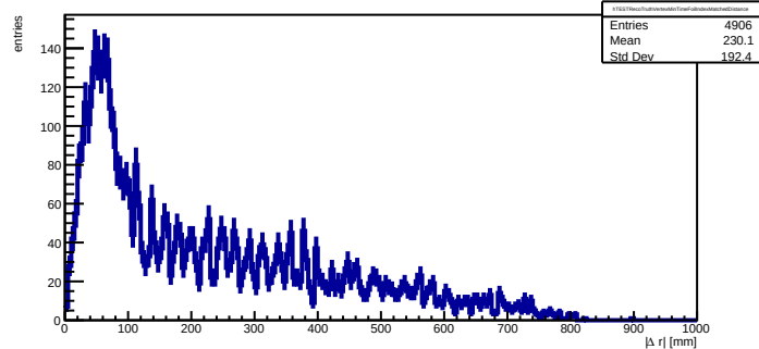
TEST: foil-index matched minimum- |\Delta t| vertex minus truth origin residual magnitude
