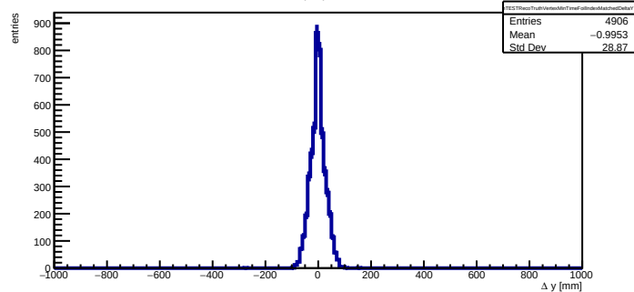
TEST: foil-index matched minimum- |\Delta t| vertex minus truth origin y difference
