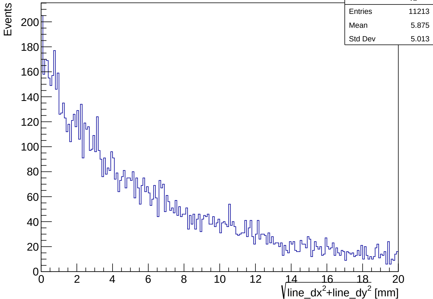
TEST: event-level closest shared ST_Foils transverse separation
