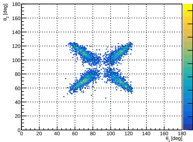
Space-selected shared ST_Foils momentum polar angles
