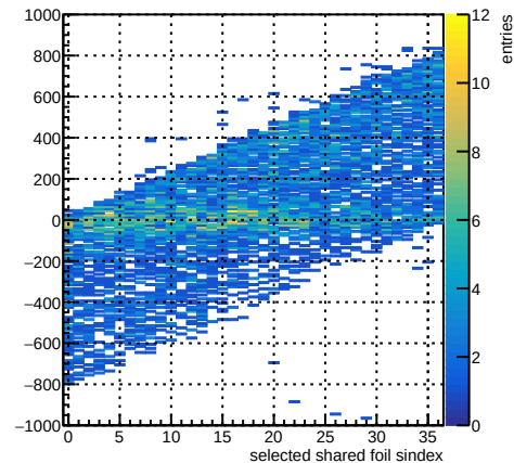
2D histogram
