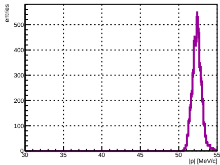
Selected track ST_Foils intersection |p|, foil index 34, N = 3879
