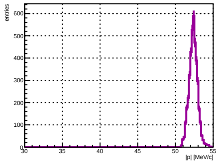
Selected track ST_Foils intersection |p|, foil index 31, N = 3939
