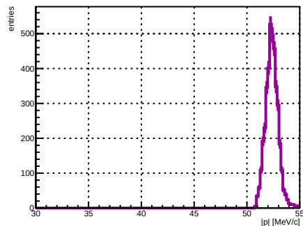
Selected track ST_Foils intersection |p|, foil index 32, N = 3965
