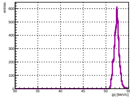
Selected track ST_Foils intersection |p|, foil index 30, N = 3977
