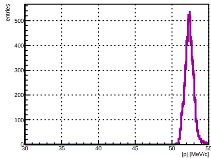
Selected track ST_Foils intersection |p|, foil index 35, N = 3871
