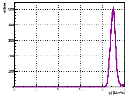
Selected track ST_Foils intersection |p|, foil index 33, N = 3965
