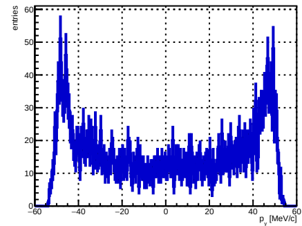
Selected track ST_Foils intersection p_y , foil index 14, N = 3580
