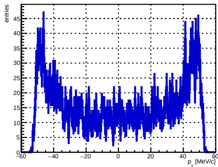
Selected track ST_Foils intersection p_y , foil index 9, N = 3466
