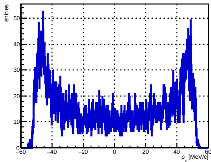
Selected track ST_Foils intersection p_y , foil index 10, N = 3430
