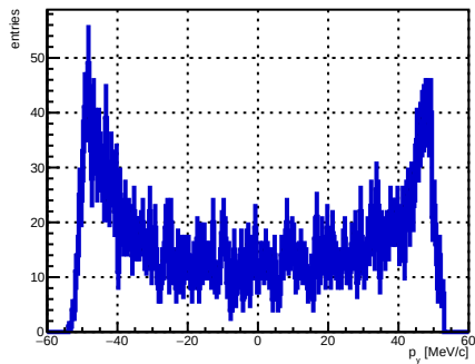
Selected track ST_Foils intersection p_y , foil index 16, N = 3644
