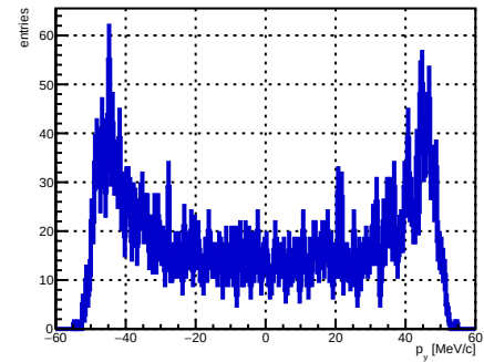
Selected track ST_Foils intersection p_y , foil index 32, N = 3965
