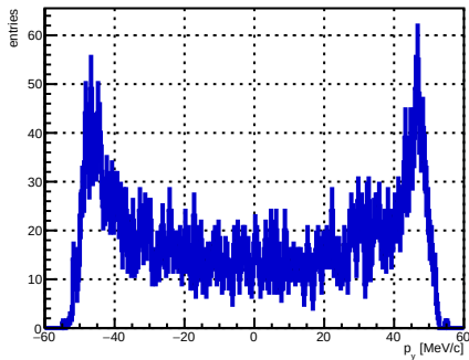
Selected track ST_Foils intersection p_y , foil index 27, N = 3985
