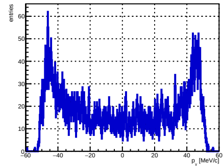
Selected track ST_Foils intersection p_y , foil index 29, N = 3933
