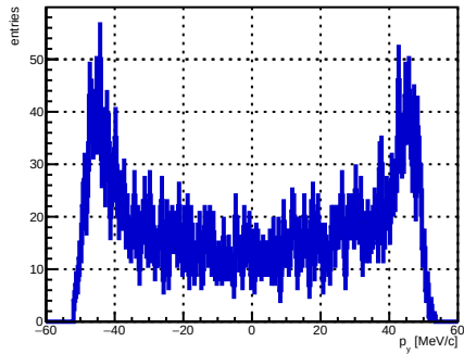
Selected track ST_Foils intersection p_y , foil index 34, N = 3879
