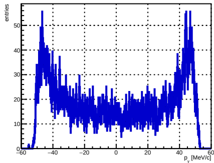
Selected track ST_Foils intersection p_y , foil index 28, N = 4058
