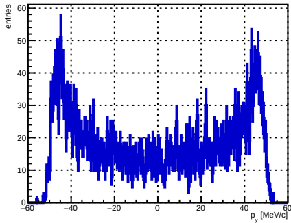
Selected track ST_Foils intersection p_y , foil index 33, N = 3965
