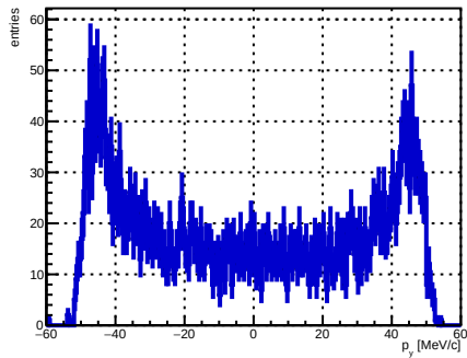
Selected track ST_Foils intersection p_y , foil index 31, N = 3939
