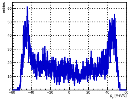
Selected track ST_Foils intersection p_y , foil index 30, N = 3977
