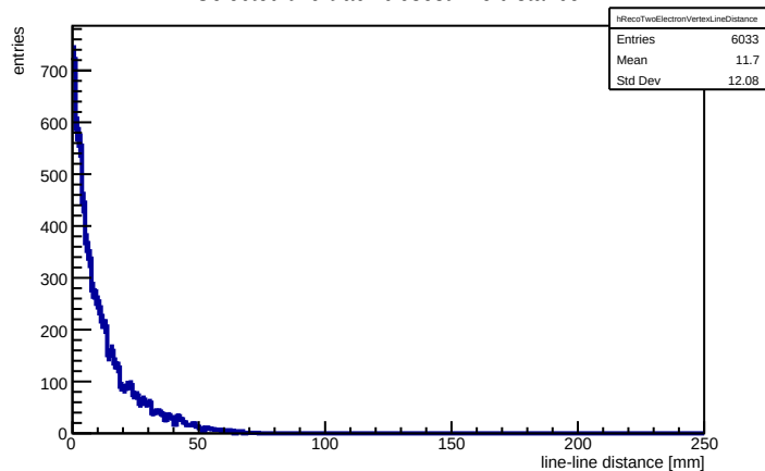
Selected two-track closest-line distance
