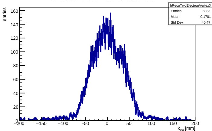
Selected two-track reconstructed vertex x
