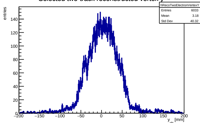
Selected two-track reconstructed vertex y
