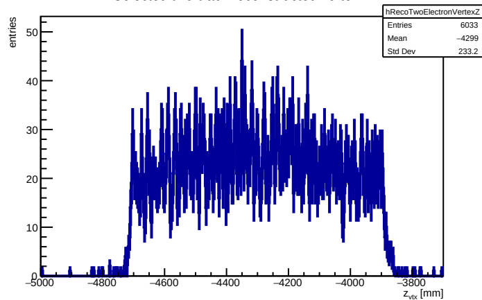
Selected two-track reconstructed vertex z
