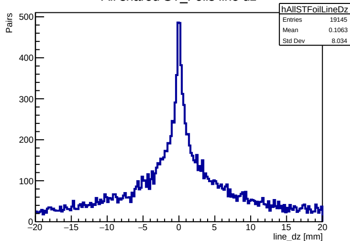
All shared ST_Foils line dz
