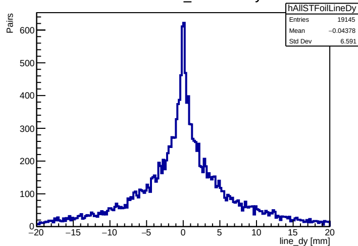
All shared ST_Foils line dy
