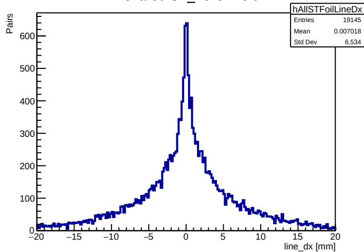
All shared ST_Foils line dx
