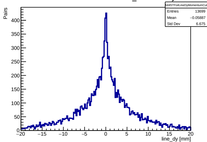
Momentum cut: all shared ST_Foils line dy
