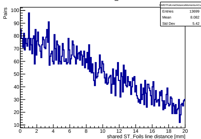
Momentum cut: all shared ST_Foils line distances
