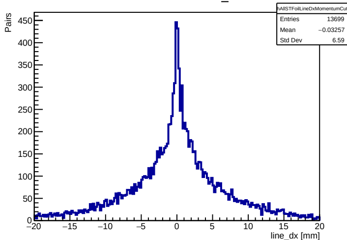
Momentum cut: all shared ST_Foils line dx
