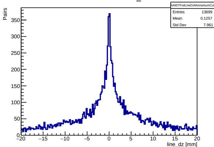
Momentum cut: all shared ST_Foils line dz
